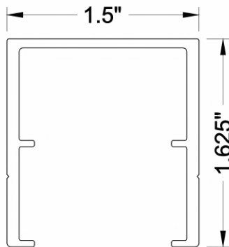
INDUSTRIAL RAIL with 1" PICKET
